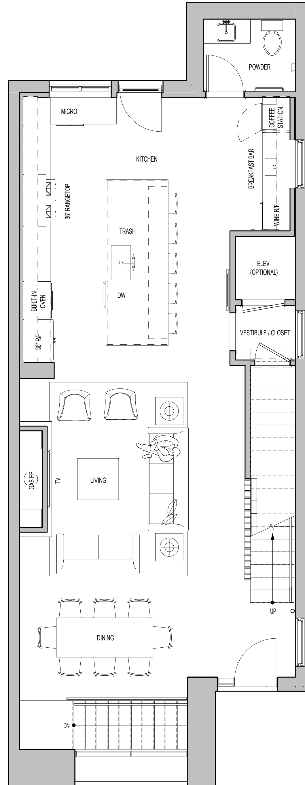
2 FIRST FLOOR PLAN 1/4" = 1'-0"
