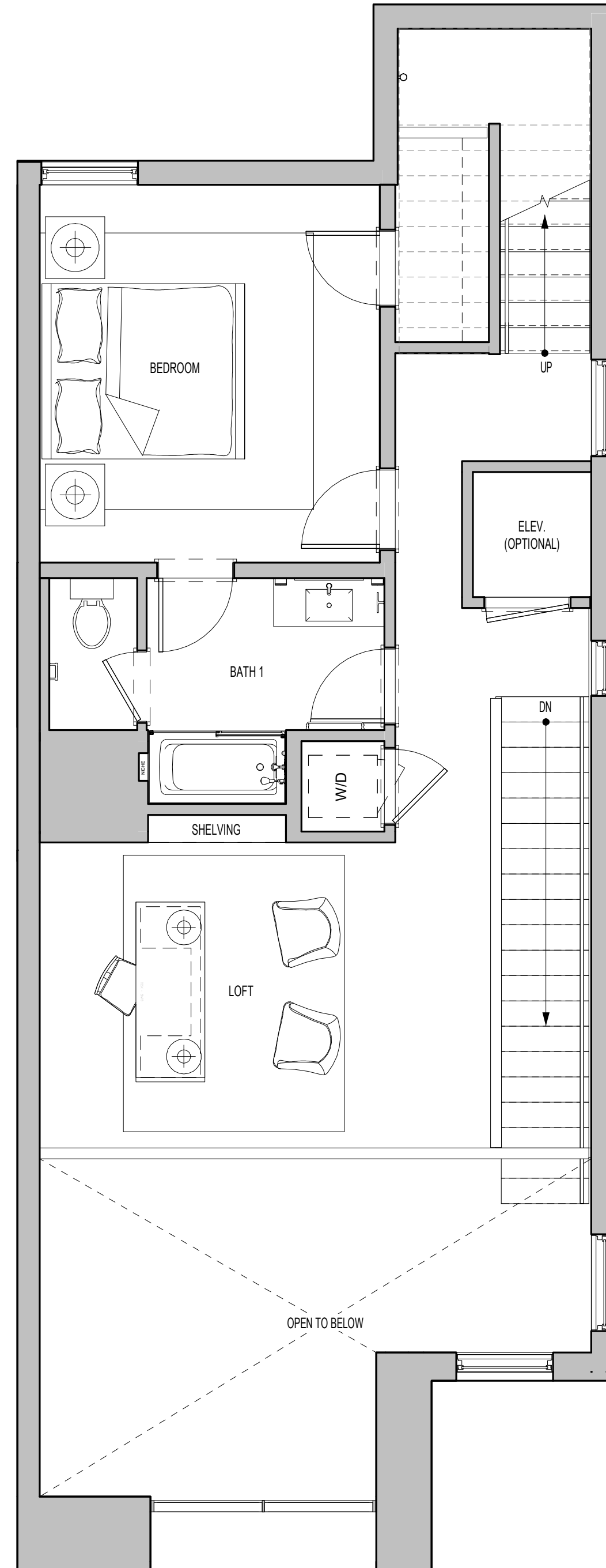
3 SECOND FLOOR PLAN 1/4" = 1'-0"
